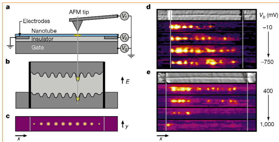
Figure 1 Scanning-gate potential imaging (SGPI) along a semiconducting carbon nanotube. a , SGPI measurement set-up. Variable bias voltages, V_b , and a gate voltage, V_g , of -6 V are applied to the TUBEFET device. An atomic-force microscope (AFM) tip at 500 mV is scanned at a constant height of about 10 nm above the surface by retracing each line taken in regular tapping mode AFM while setting a certain height offset and the cantilever amplitude to zero. b , Potential landscape of the device. In the conducting state, the valence band edge is horizontal and pinned to the edge of the Fermi level of the electrode 1,9 . The tip voltage creates a potential dip (yellow) which provides a probe for the local potential. SGPI measurements ( d,e ) show that the band edge of the nanotube is not smooth but strongly modulated. c , Corresponding SGPI measurement. The device current (colour) is displayed as a function of tip position. Current is reduced when the AFM-tip-induced barrier aligns with minima in the original potential profile. The spatial resolution of the SGPI measurements, which we estimate to be of the order of 10 nm, is determined by the tip-sample distance and the tip radius. d , AFM image of the first sample and the corresponding SGPI images for V_b values of -10 , -100 , -500 and -750 mV (top to bottom). The sample consists of an individual single-wall carbon nanotube (horizontal line) on top of two 25-nm-high platinum electrodes (on the left and right) that are spaced by 650 nm. e , AFM image of a second sample and the corresponding SGPI images for V_b values of 400, 500, 700 and 1,000 mV (top to bottom). The sample consists of an individual single-wall carbon nanotube on top of two 750-nm-spaced gold electrodes. The electrodes of this sample are embedded in the \text{SiO}_2 substrate to create a flat surface 5 (see a ).
